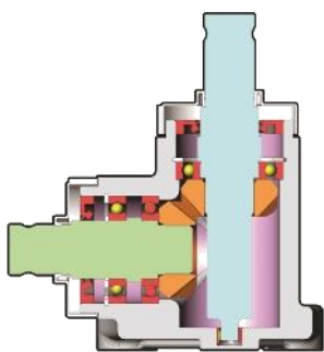
DIRECT TYPE
