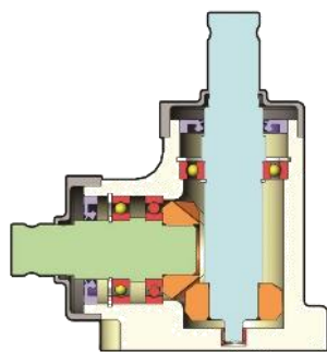
REVERSE TYPE
